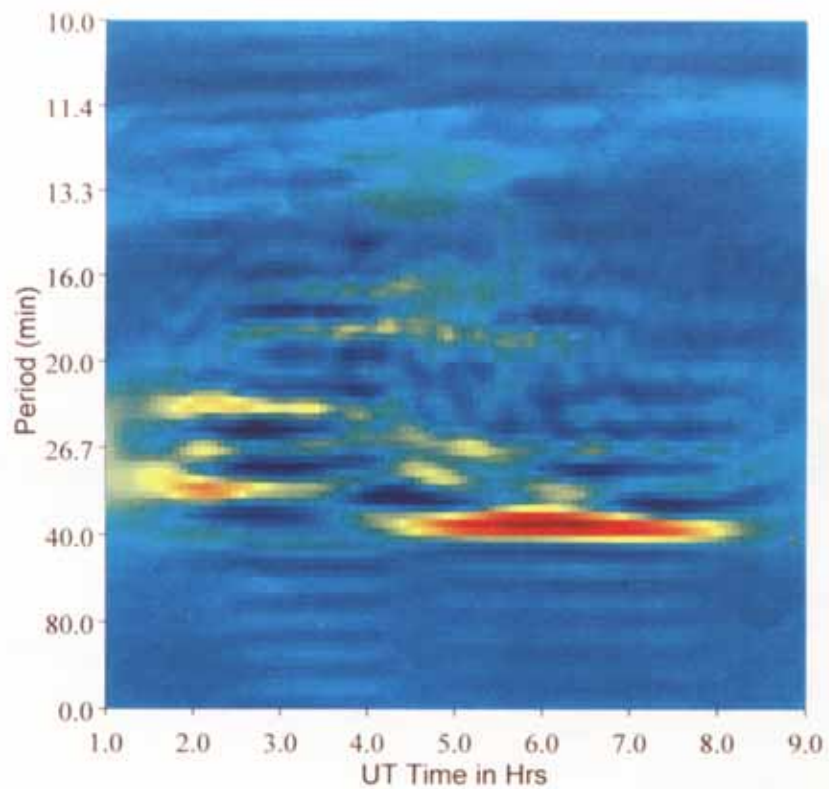
Fig. 6. WVD spectrum of the virtual height profile with time (at 4.5 MHz) on the previous control day.
