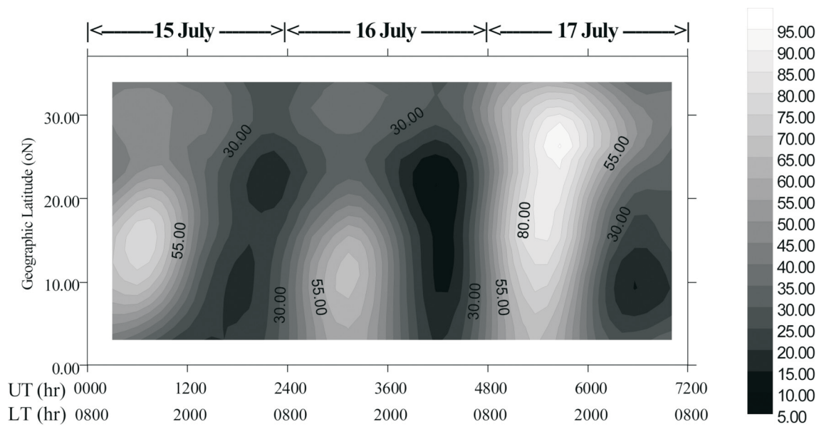
Fig. 3. TEC-Latitude-Time plots examined during 15 - 17 July 2000.
